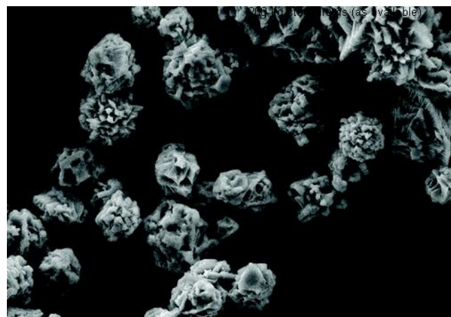
High resolution SEM image of Chemical Grade Nickel Powder
